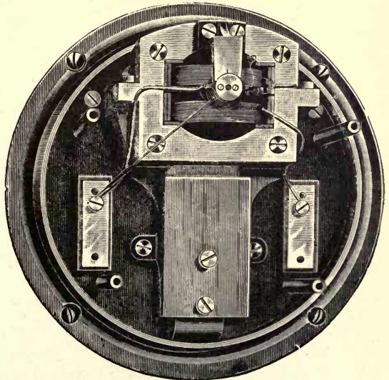
Fig. 196.—Interior, with Cover and Scale off
